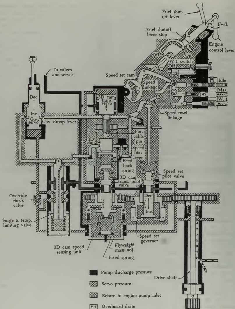
FIGURE 3-51. Scheduling system.
